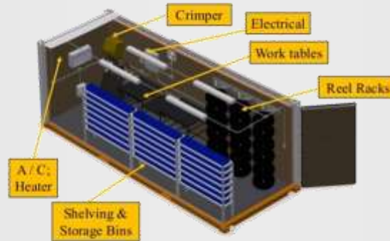
Sample Layout
